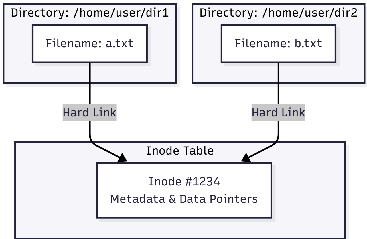
Photo: Schema of Hard Links. Two separate directory entries, a.txt in dir1
